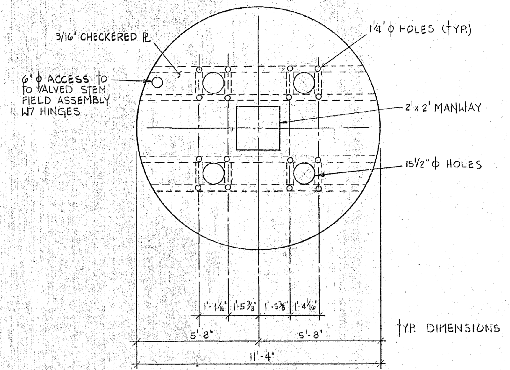
BOLT HOLE LOCATIONS
