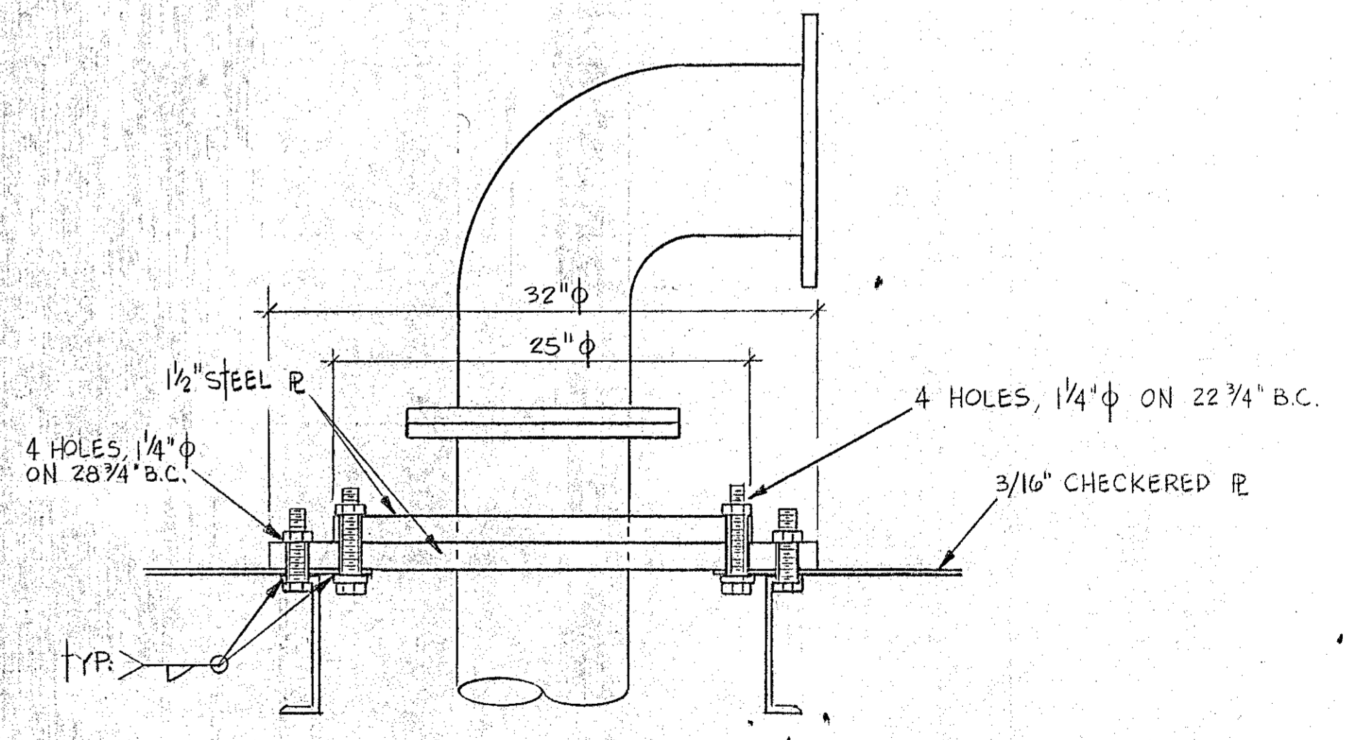
DISCHARGE HEAD
