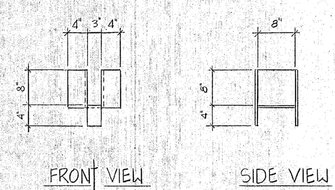
SUPPORT SADDLE
