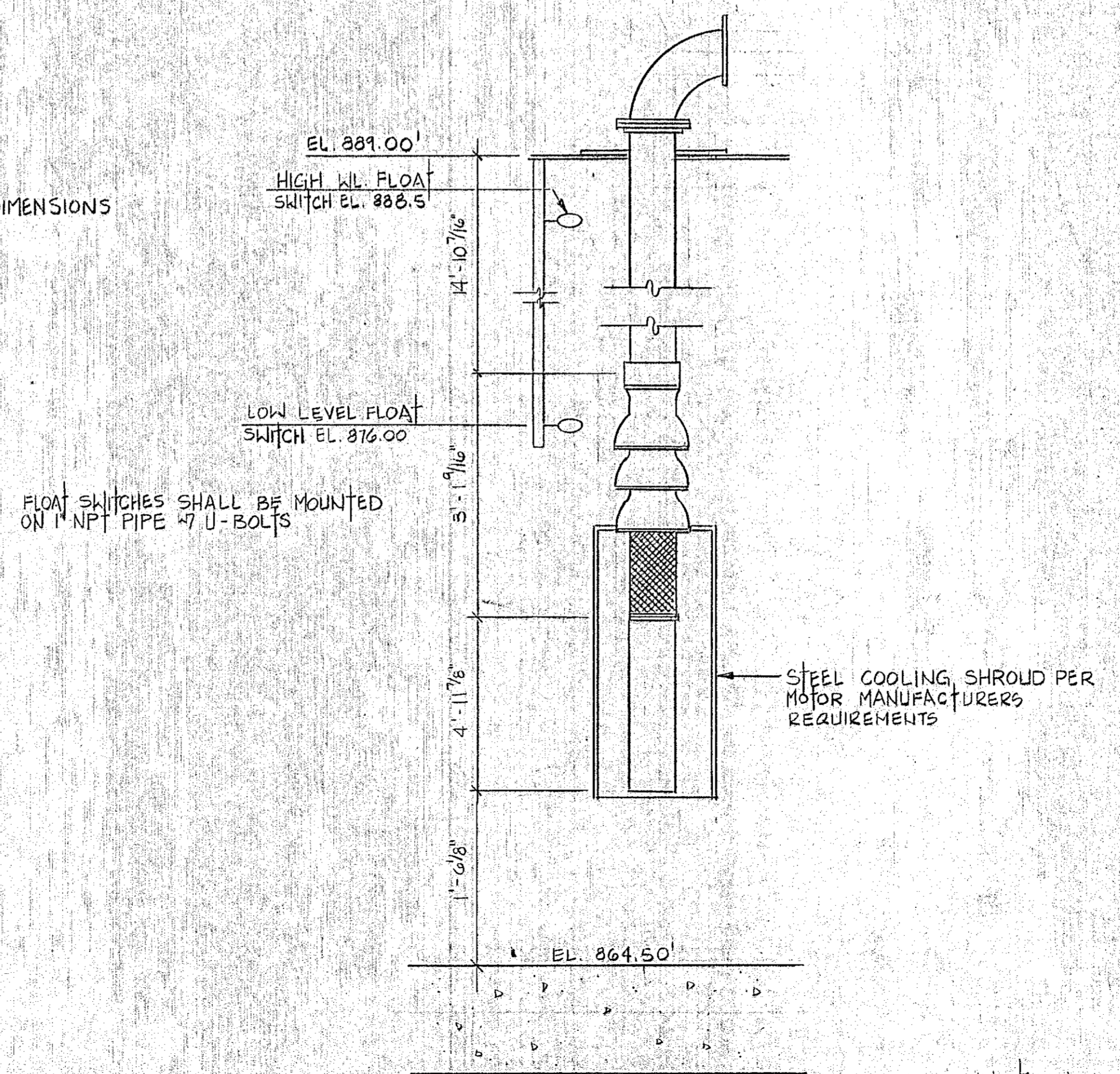
WET WELL DETAILS
